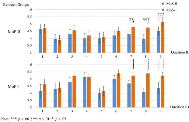
Fig. 11: MoP-0×MoS & MoP-1×MoS grading on the questionnaire, presenting mean value and standard error of each item. MoS successfully changed participants' grades on Q(7)~Q(9), regardless of different levels of Psi.
