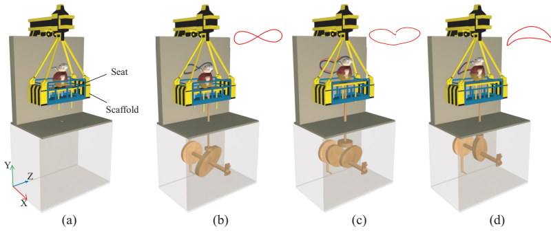
Figure 9: Effect of motion editing on the generated assembly. (a) Input. (b,c,d) Assemblies generated for different target trajectories (red curves). In each image, the blue curve on the wall shows the trajectory actually traced out by the character in the scaffold, as driven by the assembly, to match this target.
